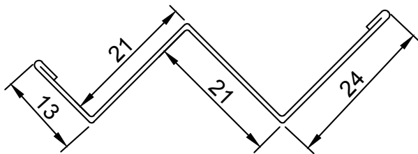
SHADOWLINE PLASTER WALL ANGLE 13 x 21 x 21 x 0.5mm
