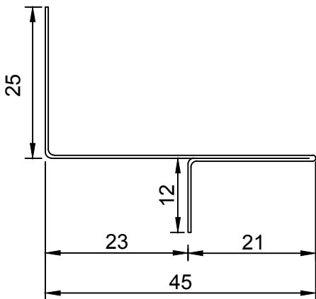
SHADOWLINE PLASTER TRIM 25 x 45 x 0.5mm
